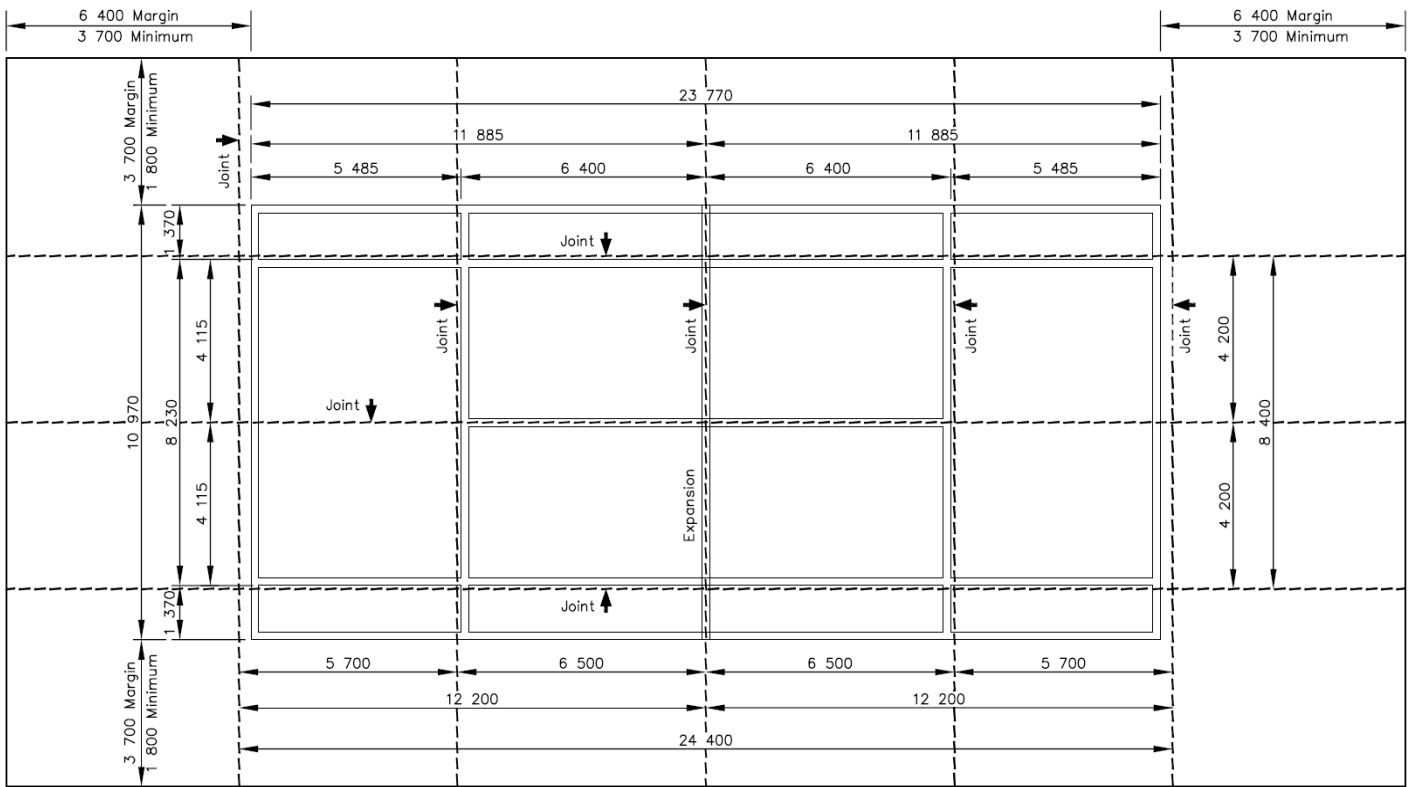
Figure 3: Layout of joints and markings
