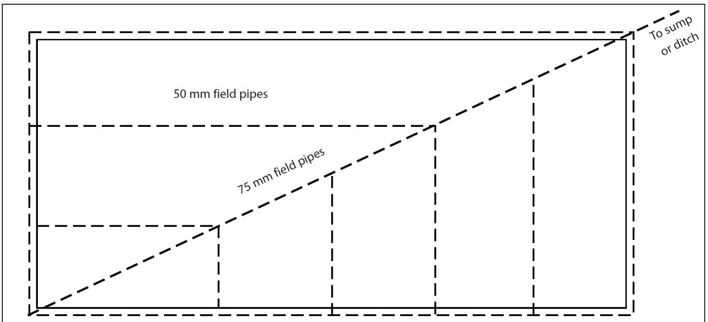
Figure 1: Drainage plan
