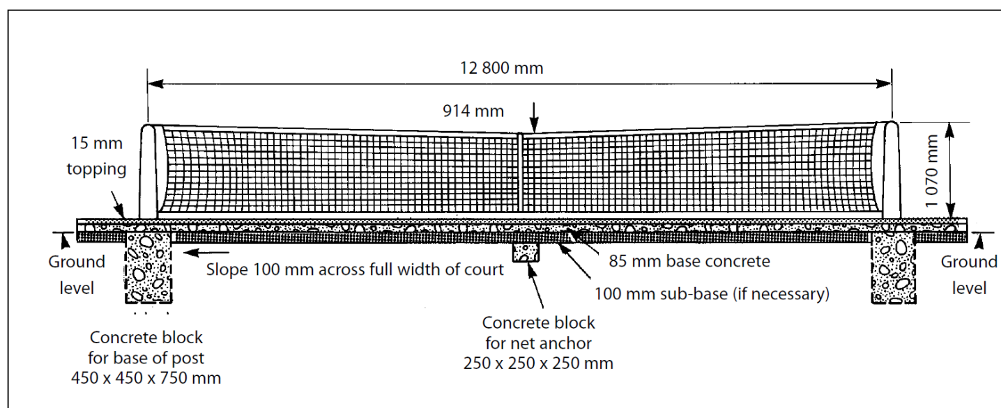
Figure 2: Cross section
